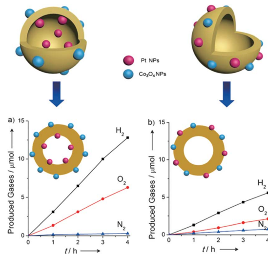
Fig. 13 Time course of the photocatalytic evolution of H 2 and O 2 using (a) Co 3 O 4 /HCNS/Pt and (b) (Co 3 O 4 + Pt)/HCNS under UV irradiation (λ > 300 nm). Reprinted with permission from ref. 40. Copyright 2016, Wiley-CVH.
