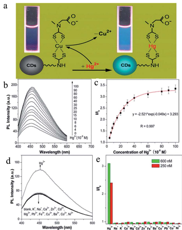
Fig. 7 (a) Schematic illustration of turn-on fluorescence nanosensor used to detect Hg 2+ ions by the Hg 2+ -induced displacement of Cu 2+ ions in a surface-bound CuDTC 2 complex. (b) Fluorescence enhancement of a solution of the CuDTC 2 -CDs probe (10 μg mL -1 ) upon the addition of Hg 2+ ions. (c) Plot of fluorescence enhancement as a function of the Hg 2+ concentration. I_0 and I represent the fluorescence intensity of the solution of the CuDTC 2 -CDs probe in the absence and presence of Hg 2+ ions, respectively. (d) Fluorescence responses of the solution of the CuDTC 2 -CDs probe (10 μg mL -1 ) in the presence of various metal ions. The concentrations of all metal ions were 150 nM. (e) Fluorescence enhancement ( I/I_0 ) of the CuDTC 2 -CDs probe after the addition of metal ions at concentrations of 250 nM and 600 nM, respectively. I_0 and I represent the fluorescence intensity of the solution of the CuDTC 2 -CDs probe in the absence and presence of metal ions, respectively. (Reprinted with permission from ref. 86. Copyright 2013, American Chemical Society.)
