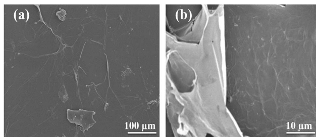
Fig. 1 SEM micrographs of graphene oxide sheets.
