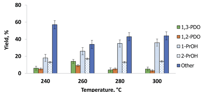
Fig. 4 Glycerol hydrogenolysis product distribution.
