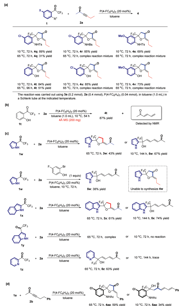
Scheme 3 Substrate containing substituents with different acidities.
