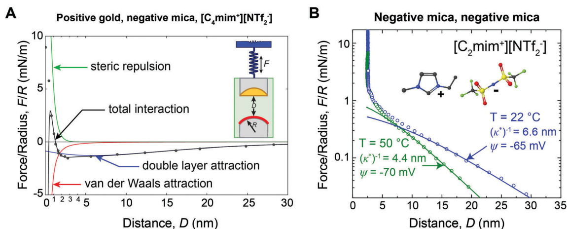
Fig. 1 (A) SFA force-distance profile between a positive gold electrode ( \Delta U = +360 mV vs. OCP) and a negative mica surface across [C_4mim^+][NTf_2^-] . Data points are equilibrium forces when bringing together the surfaces. Solid lines are fitted interaction potentials, where the total interaction (black) is a superposition of long range Poisson–Boltzmann (PB) double layer attraction (blue), short range mica–gold van der Waals attraction (red) and short range steric repulsion (green). The double layer force exhibits a decay length of (\kappa^*)^{-1} = 10 \pm 2 nm (eqn (3)). (B) SFA measurements between two negative mica surfaces across [C_2mim^+][NTf_2^-] at room temperature ( T = 22 °C) and at T = 50 °C. Data points are equilibrium forces on approach, and solid lines are fitted PB interaction potentials (eqn (2) and (3)). As the temperature is increased, (\kappa^*)^{-1} decreases, consistent with the thermal disruption of electrostatic correlations and/or effective dissociation of ionic liquid ions. Figure panel (B) reprinted from M. A. Gebbie, H. A. Dobbs, M. Valtiner, and J. N. Israelachvili, Proc. Natl. Acad. Sci. U. S. A. , 2015, 112 , 7432–7437.
