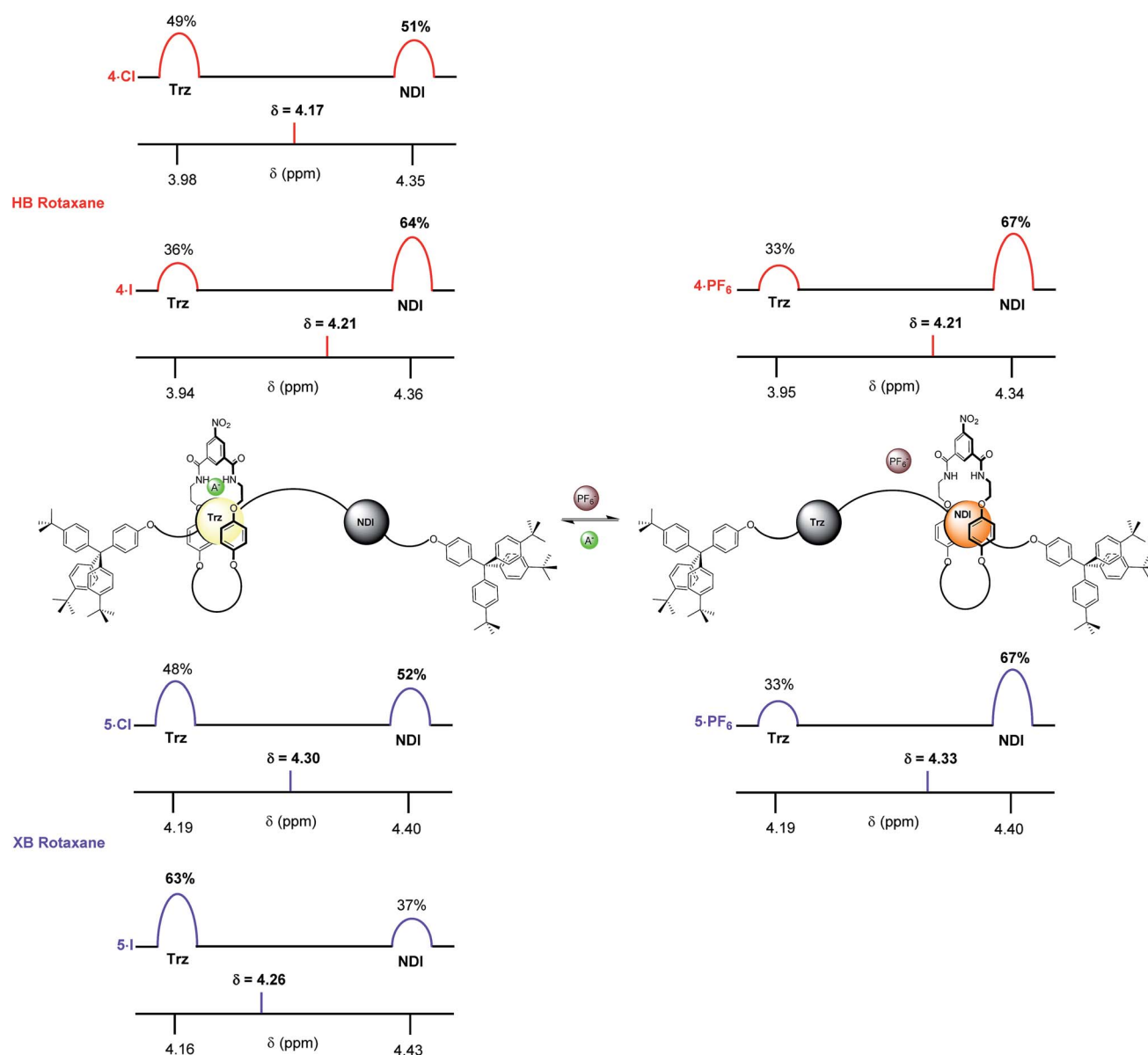
Fig. 9 The estimated percentage occupancies (based upon H 1 protons) of the HB and XB rotaxanes 4 ·A and 5 ·A as iodide and PF 6 − salts as determined by 1 H NMR spectroscopy in 1 : 1 CDCl 3 : CD 3 OD solution. A − = Cl − or I − and Trz = triazolium.
