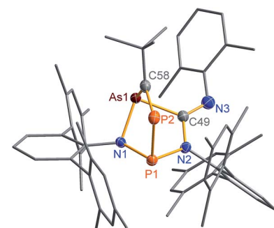
Fig. 3 Molecular structure of 3PAs . Thermal ellipsoids are drawn at 50% probability (173 K). Selected bond lengths [Å] and angles [°]: 3PAs : As1–N1 1.895(2), As1–C58 1.996(2), As1–C49 2.007(2), P1–N1 1.7378(18), P1–N2 1.756(2), P1–P2 2.2822(8), P2–C58 1.673(2), N3–C49 1.270(3), N1–As1–C58 93.47(9), C58–P2–P1 96.42(8), P1–P2–C58–As1–2.50(13).
