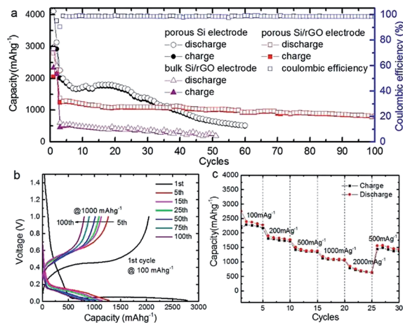
Fig. 15 (a) Cycle performance at a constant current rate of 1000 \text{ mA g}^{-1} after initial activation processes at 100 \text{ mA g}^{-1} for two cycles; (b) galvanostatic discharge–charge profiles; and (c) rate performance of Si/graphene composite electrode. 171 Reprinted (adapted) with permission from ref. 171. Copyright (2015) American Chemical Society.
