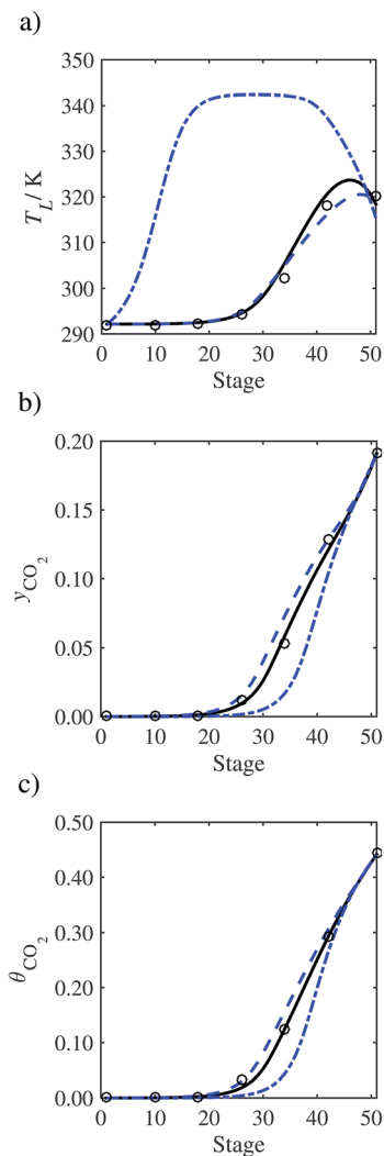
Fig. 24 Sensitivity analysis of the enthalpy of vaporization of water on the profiles predicted by our model compared with the experimental pilot-plant data of Run T22 of Tontiwachwuthikul et al. 13 Nominal value (continuous curve), enthalpy doubled (dashed curve), and enthalpy halved (dot-dashed curve). (a) Temperature profile for the liquid phase, (b) gas-phase CO 2 concentration profile, and (c) liquid-phase CO 2 loading.
