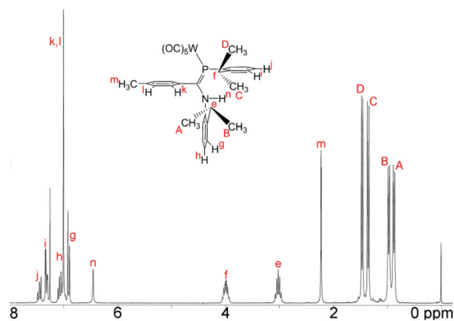
Fig. 5 1 H NMR spectrum (CDCl 3 ) of the tungsten carbonyl complex 12 . Labels indicate the assignment.
