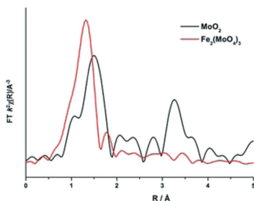
Fig. 11 Magnitude component of the k^2 weighted Fourier Transform data for \text{MoO}_2 and \text{Fe}_2(\text{MoO}_4)_3 (Sigma Aldrich).
