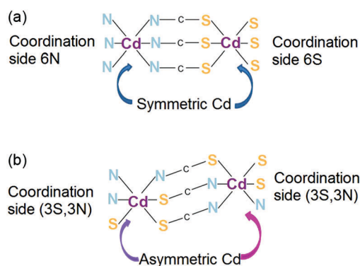
Fig. 31 Schematic representation of (a) centrosymmetric and (b) non-centrosymmetric channels of [\text{Cd}(\text{SCN})_3]^- . Adopted from ref. 118. Copyright © 2016 Elsevier B.V.
