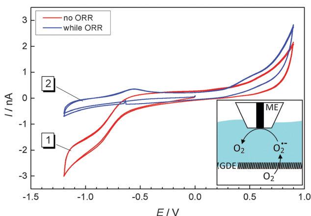
Fig. 5 CVs recorded at a ME at a distance of 10 \mu\text{m} above a GDE in 1 M LiClO 4 in DMSO; curve (1) GDE was held at OCP; curve (2) oxygen reduction at the GDE at E_{\text{GDE}} = -0.7 V. The scan rate was 100 mV s -1 . Inset: Experimental setup, oxygen from the lower gas compartment is reduced at the GDE to superoxide which diffuses towards the ME where it is oxidized/detected.
