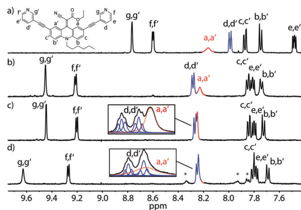
Fig. 4 ^1\text{H} -NMR spectra of (a) ligand \text{L}^{\text{Et}} , (b) cage [\text{Pd}_2\text{L}^{\text{Et}}_4] at 298 K, (c) the same cage at 333 K and (d) host-guest complex [\text{guest}@ \text{Pd}_2\text{L}^{\text{Et}}_4] containing 1.0 eq. 2,7-naphthyl bissulfonate at 333 K (400 MHz, \text{DMSO}-d_6 ). Cage formation and temperature increase leads to accelerated rotation and sharpening of the a/a' signal (red). Guest uptake slows down spinning of the endohedral rotor, as shown by line fitting analysis of deconvoluted signals d/d' (blue) and a/a' (red). * = signals of the encapsulated guest.
