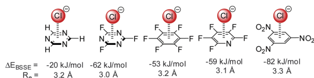
Fig. 2 Interaction energy with basis set superposition error correction ( E_{\text{BSSSE}} ) and equilibrium distances ( R_{\text{e}} ) of selected anion- \pi complexes from the MP2/6-31++G** level of theory. 7,15,16
