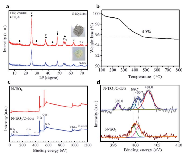
Fig. 4 (a) XRD patterns of N-TiO 2 and N-TiO 2 /C-dots composite. (b) TG analysis of N-TiO 2 /C-dots composite. (c) The survey scan of XPS and (d) N 1s core level XPS spectra of N-TiO 2 and N-TiO 2 /C-dots.
