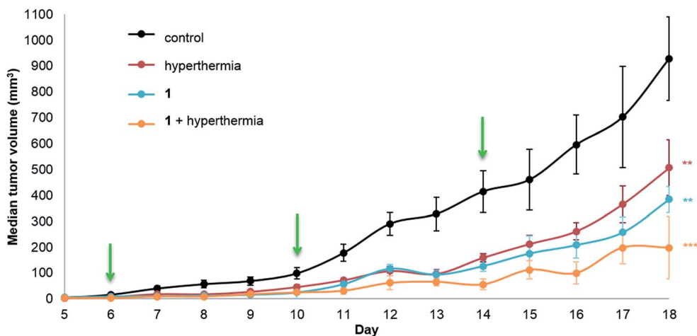
Fig. 2 LS174T adenocarcinoma growth inhibition in athymic mice. Mice were treated with 1 (12.5 mg kg -1 , 300 μL i.p.) given every 4 days (indicated by the green arrows) with or without mild hyperthermia (42 °C for 30 minutes) within 15 minutes following drug injection. The control group animals were treated with 10% DMSO in sterile saline (0.9% NaCl) also given every 4 days. Results are expressed as medians ± the standard error of the mean, SEM ( n = 5 to 8 mice/group, ANOVA, **p < 0.01 , ***p < 0.001 ), efficacy DE_{1,H} = 0.787 . Tumor volume (mm 3 ) was calculated using the formula: volume = width 2 × length × 0.5.
