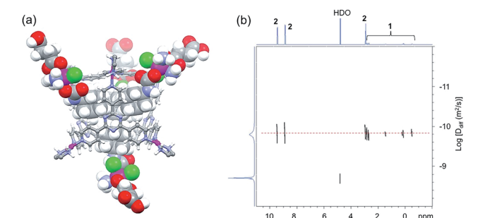
Fig. 1 (a) A 3D model of the host-guest complex 3 and (b) DOSY NMR spectrum (400 MHz, R.T.) of 3 (2.8 mM) in D 2 O ( D = 1.3 \times 10^{-10} \text{ m}^2 \text{ s}^{-1} ).
