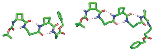
Fig. 3 Top-view of the low energy conformers of \beta/\gamma -peptides 3 (left) and 5 (right), showing the alternating C9/C8 H-bonding network.
