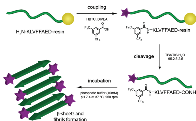
Fig. 1 Scheme of F -A \beta (16–23) synthesis and aggregation.
