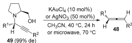
Scheme 14 A possible mechanism of the ATA reaction.
