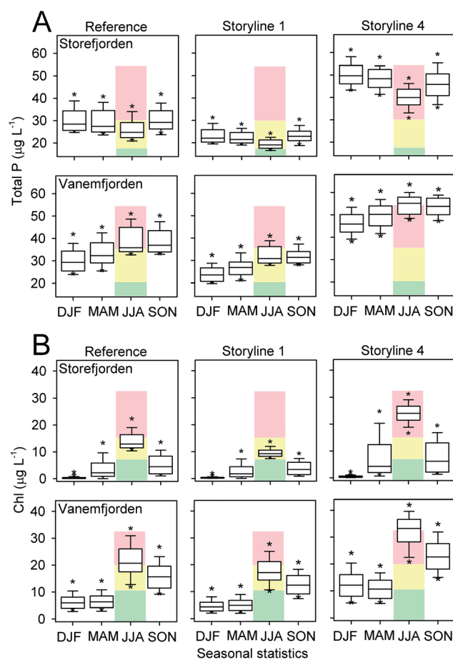
Fig. 8 Seasonal range of MyLake-predicted daily TP (panel A) and chlorophyll (panel B) concentrations in the top 4 m of the Storefjorden (L1) and Vanemfjorden (L2) water columns. The green, yellow and red shaded zones indicate the basin-specific WFD water quality targets for good, moderate and bad water quality status, respectively (see Table 4), while the asterisks indicate the 5 th and 95 th percentile outliers.
