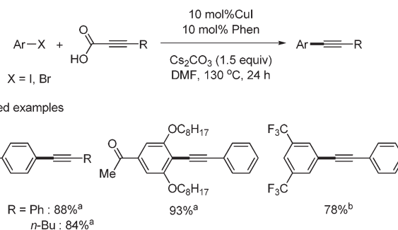
Scheme 33 Decarboxylative coupling by copper catalyst. a Yield from aryl iodide; b yield from aryl bromide.
