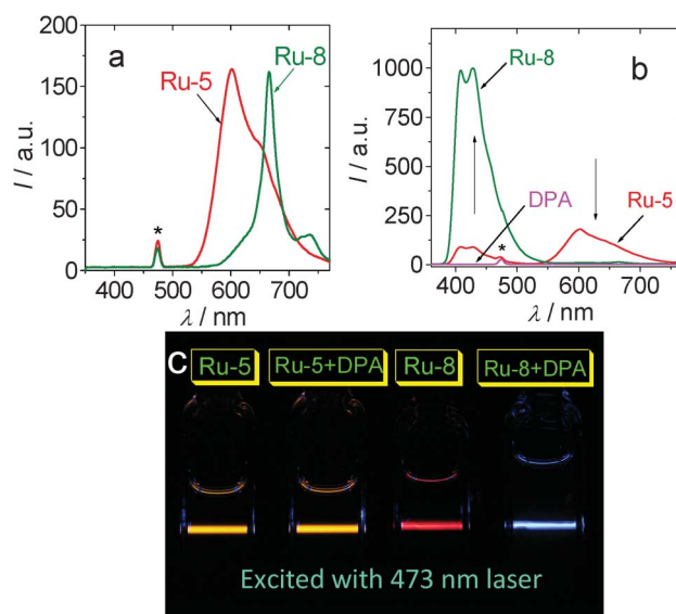
Fig. 6 Emission and upconversion of Ru-5 and Ru-8 with 473 nm laser excitation. (a) Emission of the Ru(II) complexes. Excited by blue laser ( \lambda_{\text{ex}} = 473 \text{ nm} , 5 mW). In order to show the different emission intensity of the complexes, the spectra were not normalized. (b) The upconverted DPA fluorescence and the residual phosphorescence of the mixture of DPA ( 4.3 \times 10^{-5} \text{ M} ) and Ru-5 or Ru-8 , respectively. (c) The photographs of the upconversion (samples of a and b). In deaerated \text{CH}_3\text{CN} solution. The complexes solution are 1.0 \times 10^{-5} \text{ M} . The asterisks in (a) and (b) indicate the scattered 473 nm excitation laser. 25 ^\circ\text{C} . Adapted from ref. 26 with permission.
