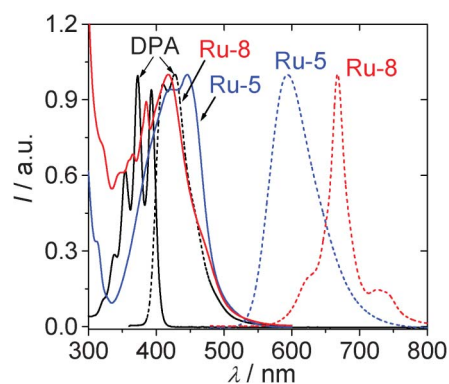
Fig. 5 Normalized absorbance (solid lines) and emission spectra (dotted lines) of DPA, Ru-5 and Ru-8 in acetonitrile ( 1.0 \times 10^{-5} \text{ M} ). DPA, \lambda_{\text{ex}} = 380 \text{ nm} ; Ru-5 , \lambda_{\text{ex}} = 446 \text{ nm} ; Ru-8 , \lambda_{\text{ex}} = 418 \text{ nm} . 25 ^\circ\text{C} . Adapted from ref. 26 with permission.
