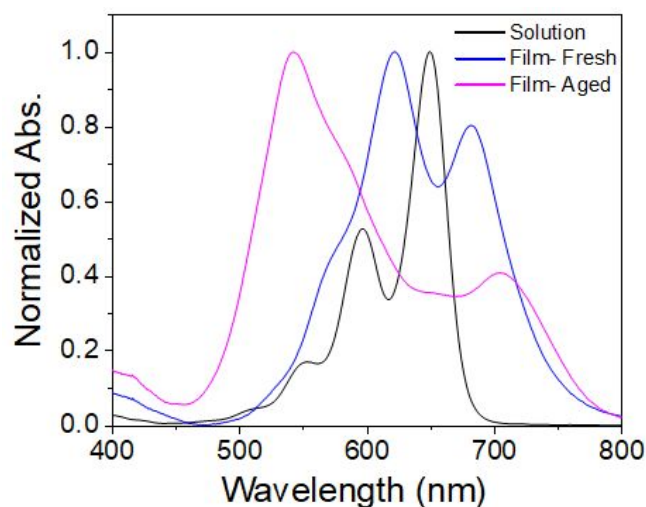
Figure 1: Steady-state absorption spectra of C 23 TDI in THF solution, (black), freshly prepared film (blue), and aged film (purple).
