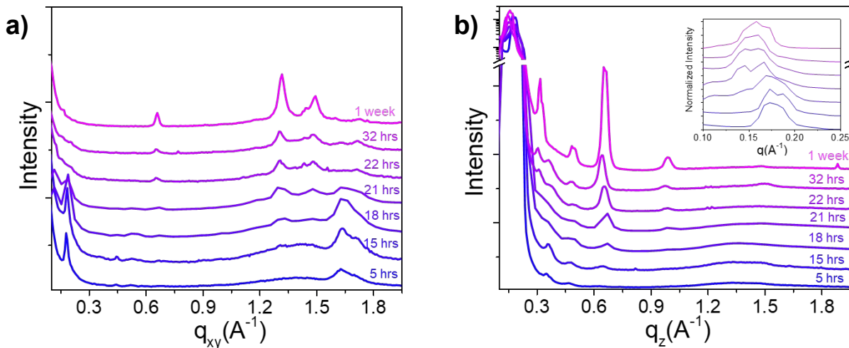
Figure 4: GIWAXS scans of C_{23}TDI Films: horizontal (a) and vertical (b) linecuts of films at various time points after film preparation. Inset shows magnified small q region.
