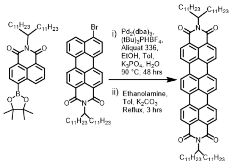
Scheme 1: Synthetic scheme for C 23 TDI
