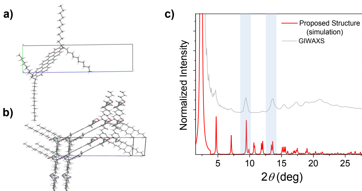
Figure 6: a) Proposed crystal structure unit cell from simulated annealing result. b) Contents of 4 unit cells ( 2 \times 1 \times 2 ), rotated to highlight crystal packing. c) Overlay of experimental GIWAXS spectrum of aged film (gray) and simulated powder patterns for simulated annealing result (red). Blue shading highlights regions of interest corresponding to (004) and (014) reflections.
