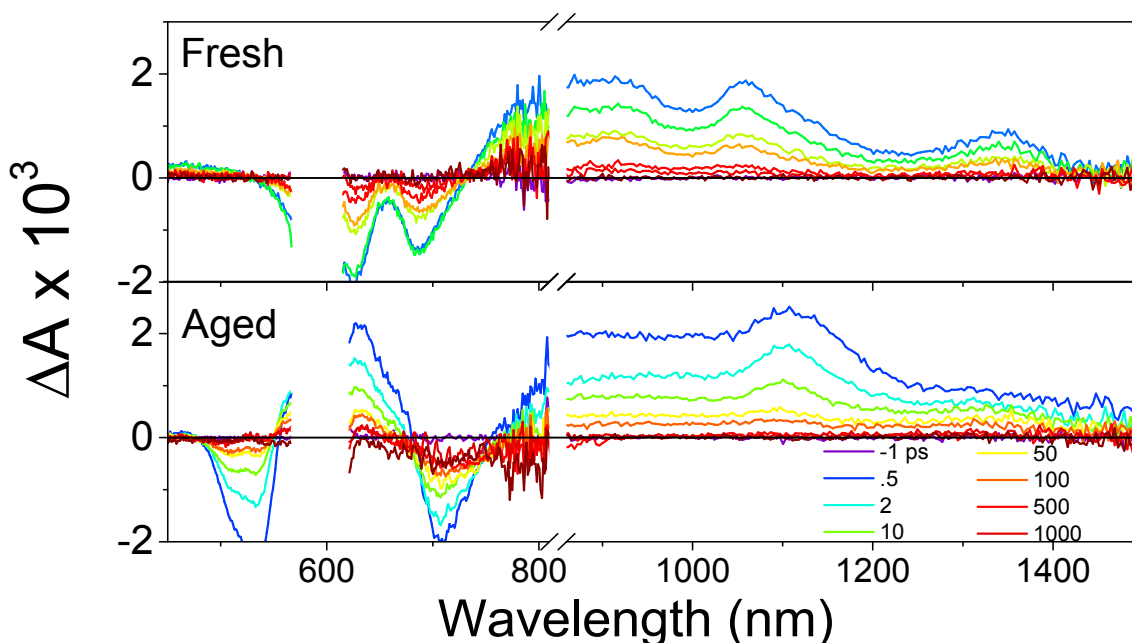
Figure 8: Transient absorption spectra at selected decay times after excitation at \lambda_{ex} = 590 nm for both fresh and aged films.
