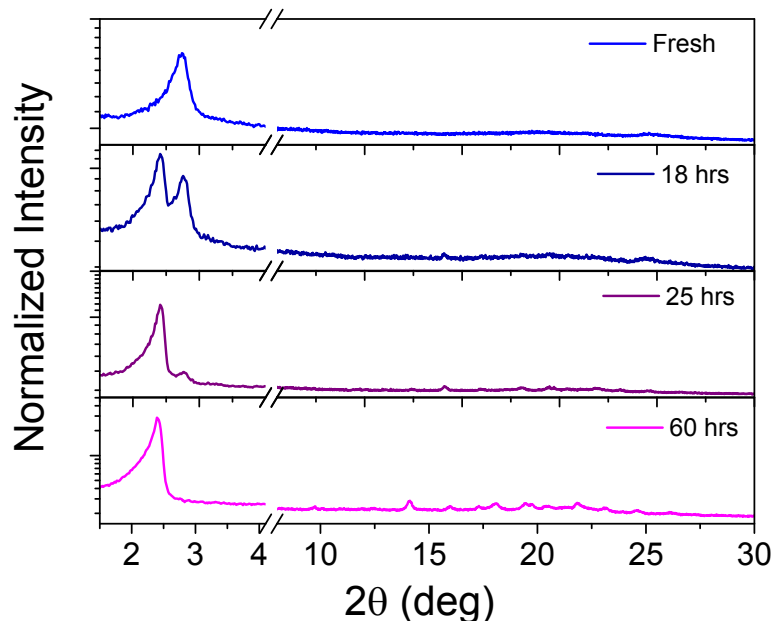
Figure 3: PXRD spectra of bulk C_{23}TDI powder, with time after solvent evaporation.
