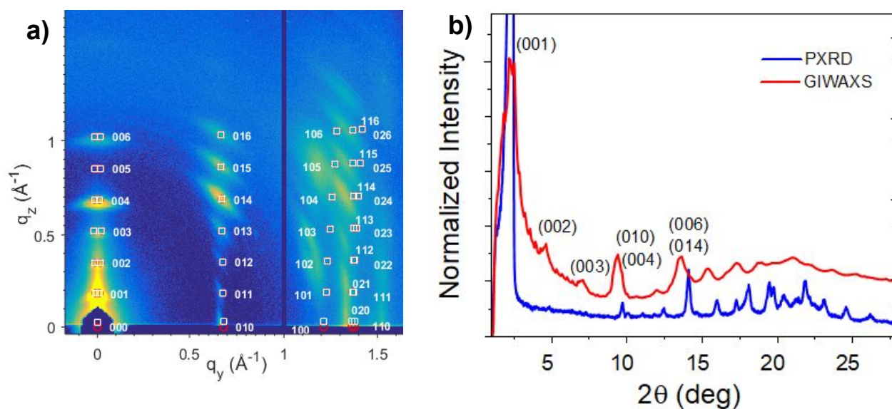
Figure 5: a) Overlay of diffraction peaks for extracted unit cell on 2D GIWAXS pattern and Miller indices. (b) Overlay of diffraction patterns of bulk powder (blue) and radially integrated line cut of GIWAXS data from film (red).
