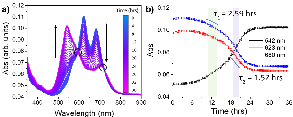
Figure 2: a) Steady-state absorption spectra of C_{23}TDI film, collected in 30 minutes increments. Isosbestic points are circled. b) kinetic traces of representative wavelengths (open squares), with fits to eq 1 (solid lines).
