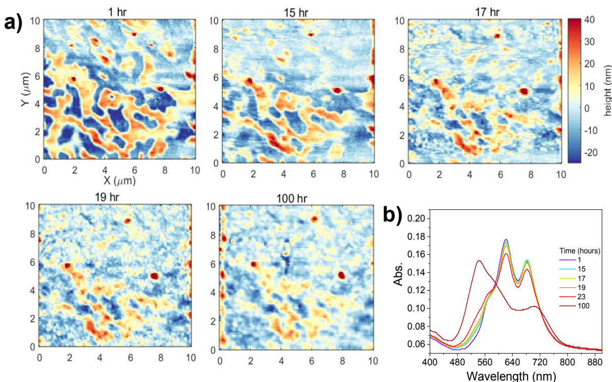
Figure 7: a) AFM topography at five time delays following film preparation. b) Visible absorption spectra of film from the same preparation at identical time intervals.
