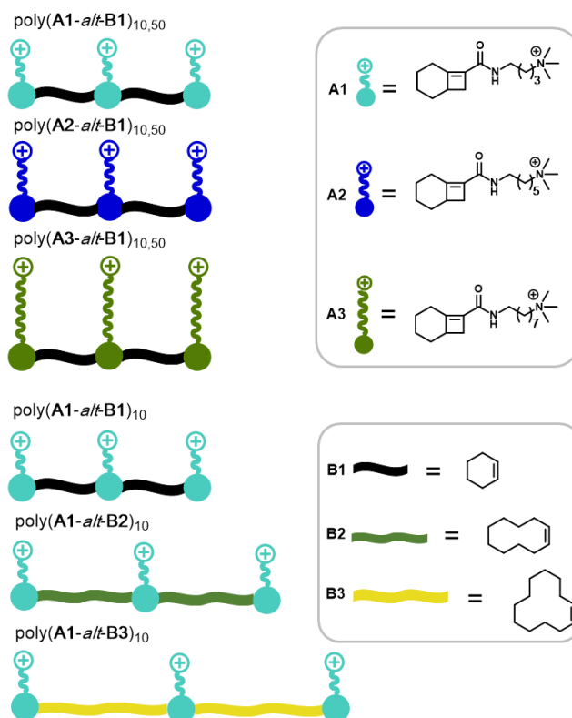
Fig. 1 Structures of monomers (before ring-opening) and polymers synthesized and characterized in this work.
