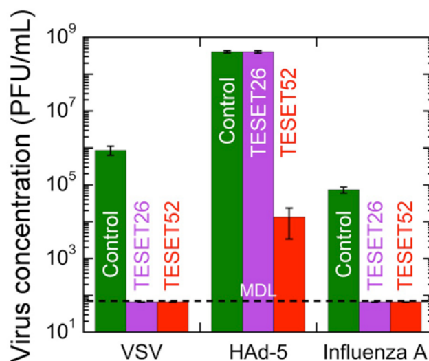
Figure 4. The infectivity of three viruses after exposure to a control (green), TESET26 (purple) and TESET52 (red) for 5 min. In the case of the two enveloped viruses, inactivation is complete (falling below the MDL of 66.7 PFU/mL).
