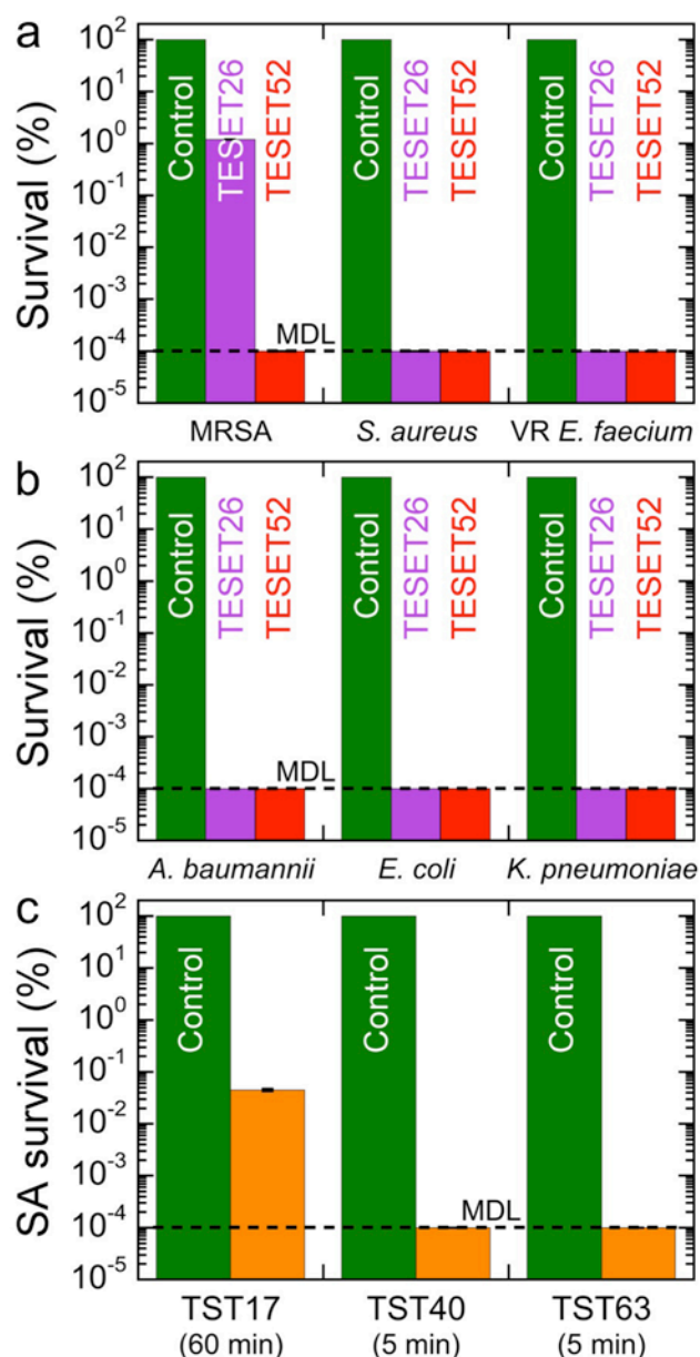
Figure 2. Survival of (a) Gram-positive and (b) Gram-negative bacteria after exposure to a control (green), TESET26 (purple) and TESET52 (red) for 5 min. In (c), the survival of methicillin-susceptible S. aureus is presented for three TST polymers varying in midblock sulfonation content (exposure times are included).
