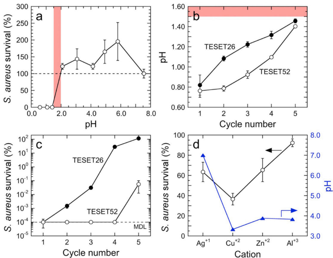
Figure 3. In (a), the survival of methicillin-susceptible S. aureus at different pH levels. The red shaded region identifies the transition below which the bacteria are killed. The pH of PBS solutions in contact with TESET26 (●) and TESET52 (○) is presented in (b) for up to five successive cycles, and the corresponding survival of S. aureus under these change pH conditions is included in (c). In (d), the effect of ion complexation on S. aureus exposed to TESET52 is compared with pH level (▲). In all cases, the solid lines serve to connect the data, and the error bars denote the standard error associated with at least triplicate measurements.
