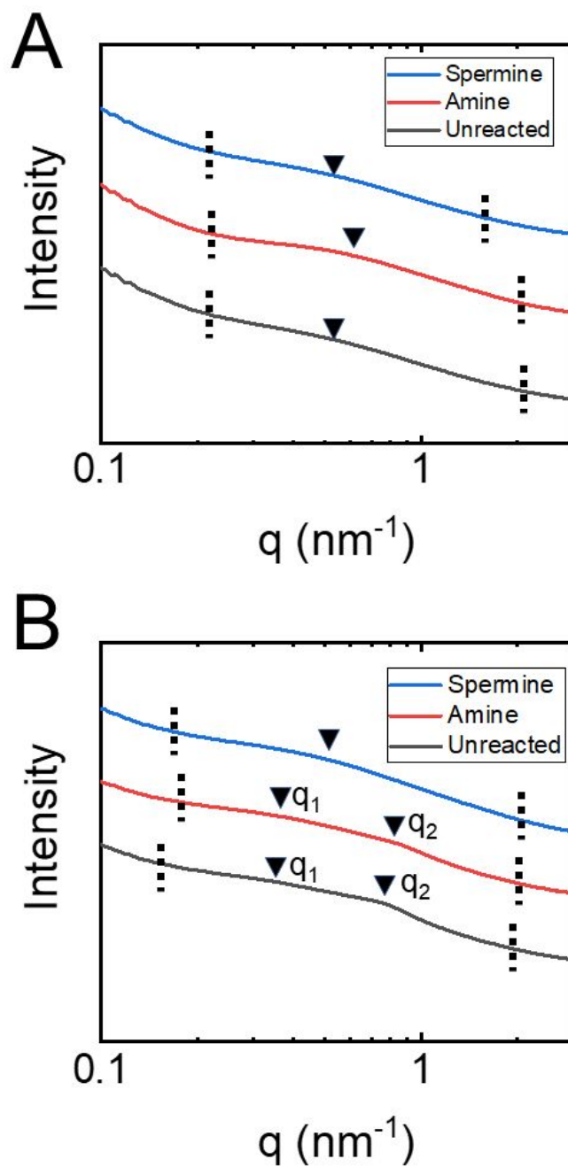
Figure 4: One-dimensional SAXS traces for P(TFEMA-OEGMA-GMA) copolymer membranes (A) in the dry state and (B) submerged in water. The dashed vertical lines indicate the region of
