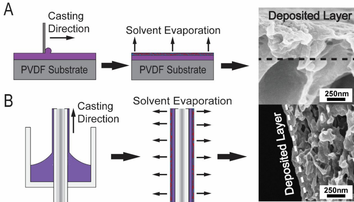
Figure 1: (A) Flat sheet membranes are blade-coated using a doctor's blade fixed at a pre-determined gate height; solvent is allowed to evaporate from the resulting thin film of solution, which drives microphase separation of the copolymer at the solution-air interface; after the evaporation period, the film is plunged into a non-solvent bath to set the membrane structure. (B) Dip-coated hollow fiber membranes are fabricated using a custom die, through which a substrate fiber is pulled. The dip-coating process results in a thin layer of copolymer casting solution being deposited on the substrate. After coating, the procedure is the similar to that used in the blade-coated method. A key distinction is the fiber is inverted during the solvent evaporation step and then submerged into the non-solvent bath at the translation velocity used for coating. This consideration ensures a uniform evaporation time over the whole length of the fiber.
