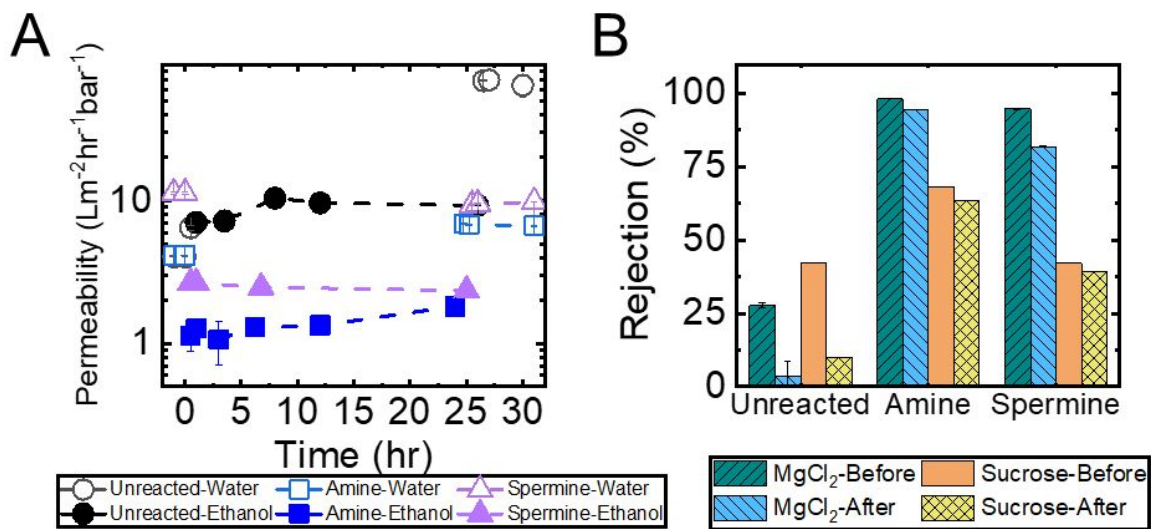
Figure 6: (A) Permeability of unreacted, diamine-functionalized, and spermine-functionalized membranes. These membranes were subjected to ethanol for approximately 24 hours and then changed to water. The time started from the moment the pressure was applied to the membrane in ethanol. The errors are one standard deviation of n=2 samples taken from one membrane. (B) Rejections of 1 mM \text{MgCl}_2 and 1 g L -1 sucrose solutions of the unreacted, diamine-functionalized, and spermine functionalized membranes before and after subjected to ethanol permeation. The errors are one standard deviation of n=2 samples from one membrane.
