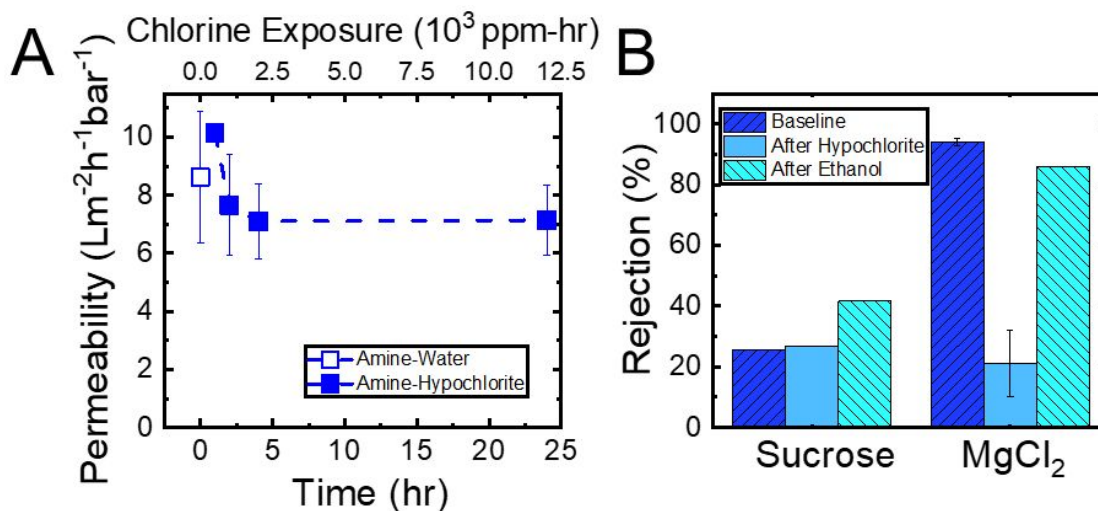
Figure 8: (A) Permeability of the amine-functionalized membranes as a function of chlorine exposure time. The membranes were subjected to an aqueous feed solution containing 500 ppm hypochlorite for 24 hours. The t=0 time point is determined by the moment when the applied transmembrane pressure stabilized in the module after switching from a DI water feed solution to a chlorine-containing feed solution. The error bars represent one standard deviation of n=2 samples. (B) 1 mM \text{MgCl}_2 and 1 g \text{L}^{-1} sucrose rejections of the amine-functionalized membranes before the membranes were exposed to the 500 ppm chlorine feed solution, after the 24-hour experiment, and after the membrane was permeated with ethanol for 6 hours. The error bars represent one standard deviation from n=2 samples.
