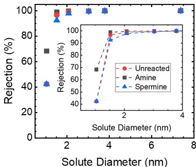
Figure 3: Neutral solute rejection curves for the unreacted, amine-functionalized, and spermine-functionalized membranes. 1 g L -1 solutions of sucrose and PEO with molar masses of 1.1, 2.1, 4.0, 6.0, and 19.0 kg mol -1 dissolved in DI water were used as feed solutions. The solute concentrations in the feed and permeate samples were analyzed using TOC analysis. These values were then used to calculate the observed sieving coefficient. Concentration polarization was accounted for using a mass transfer correlation 43 . The error bars, which are smaller than the symbols, represent one standard deviation from n=2 samples taken using the same membrane.
