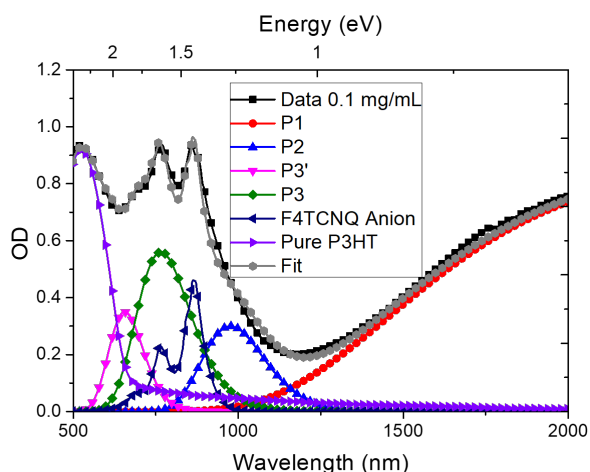
Fig. 12 Reconstruction of the absorption spectrum of a P3HT film sequentially doped with a 0.1 mg/mL solution of F4TCNQ in DCM using a linear combination of the known F4TCNQ anion spectra (taken from Wang et al. ), 33 the known spectrum of neutral P3HT (Fig. 1), and the Gaussian fits of the peak positions of the fast component (which we assign to free polarons) extracted from the global model of our transient absorption measurements (Table 1); see text for details. The excellent agreement between the measured spectrum and the reconstructed fit shows that our transient absorption measurements, global fit, and steady-state absorption measurements are all internally consistent.
