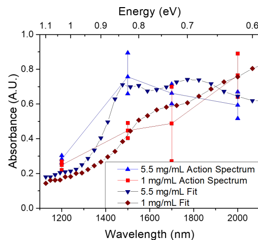
Fig. 11 The action spectra of trapped polarons from Fig. 10 fit to linear combinations of the anion-distance-dependent P1 spectra calculated by Spano and co-workers shown in Fig. 3. 23 The 5.5 mg/mL F4TCNQ-doped P3HT film (blue triangles) fits best to a sum of the theoretical spectra with anion distances calculated for 0.2, 0.4, and 0.6 nm spacing between the anion and the polymer chain with 20, 7, and 73% relative weightings, respectively. The 1 mg/mL F4TCNQ-doped P3HT film (red squares) fits best to a sum of the spectra for anion distances calculated for 0.4, 0.6, and 0.8 nm spacing between the anion and the polymer chain with 6, 4 and 90% relative weightings, respectively.
