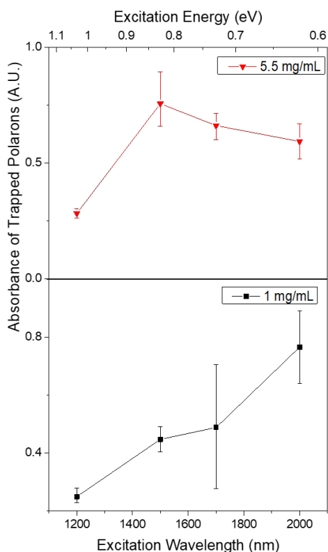
Fig. 10 The calculated action spectrum of trapped polarons for: a) a P3HT film sequentially doped with a 5.5 mg/mL F4TCNQ solution, and b) a P3HT film sequentially doped with a 1 mg/mL F4TCNQ solution. This spectrum was calculated by scaling the measured ratios of the slow to fast components in Fig. 9 by the absorption of a P3HT film sequentially doped with a 0.1 mg/mL F4TCNQ solution, which we expect has few trapped polarons. The data make clear that the more highly-doped sample has trapped polarons with a more blue-shifted absorption spectrum, indicating that these polarons are more highly trapped than those in the lower-doped sample.
