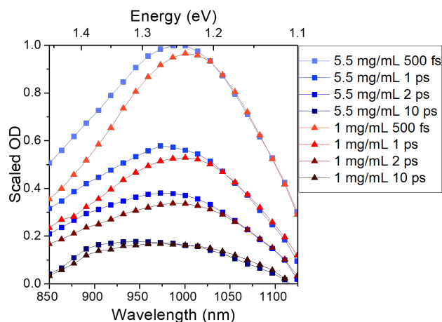
Fig. 7 Ultrafast transient absorption spectra of P3HT films that have been sequentially doped either with a 1 mg/mL solution of F4TCNQ in DCM (red triangles) or a 5.5 mg/mL solution of F4TCNQ in a 70:30 v:v mixture of THF:DCM (blue squares) following excitation at 1200 nm. Data are shown for 0.5, 1, 2, and 10 ps delays between excitation and collection, with darker colors corresponding to later delay times. The more highly-doped samples have the transient absorption shifted to the blue and the blue feature decaying more slowly than the lower-doped sample.
