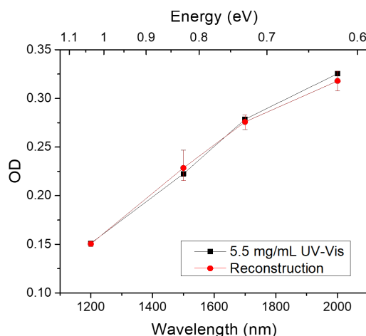
Fig. 13 Reconstruction of the absorption spectrum of a highly-doped P3HT film (created using a 5.5 mg/mL solution of F4TCNQ). The reconstructed spectrum uses the spectrum of a low-doped P3HT film (created using an 0.1 mg/mL F4TCNQ solution) and the action spectrum of trapped polarons that we extracted from the ultrafast transient absorption data in Fig. 10; see text for details. The excellent agreement provides confirmation that the action spectrum taken from our ultrafast measurements can be used to account for the spectral shape changes observed between the high- and low-doped P3HT films seen in Fig. 1.
