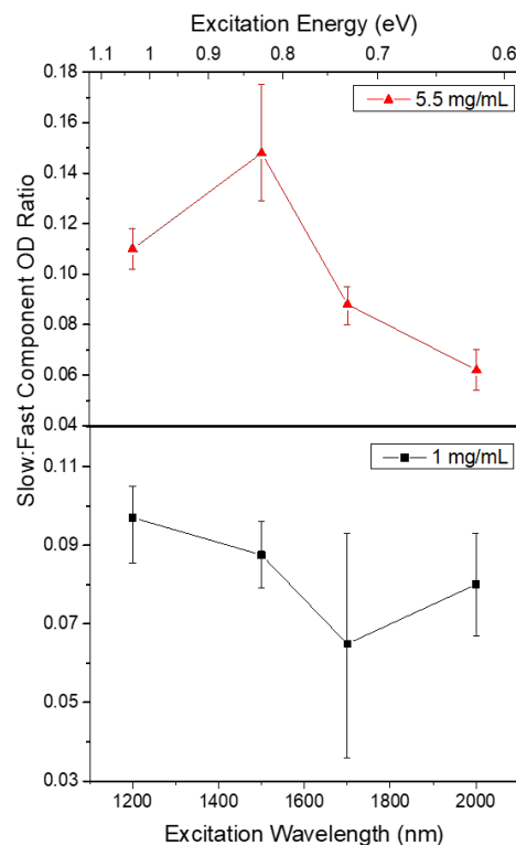
Fig. 9 The ratio of the initial optical densities of the extracted slow to fast components from the global fit of the transient absorption measurements as a function of excitation wavelength for: a) a P3HT film sequentially doped with a 5.5 mg/mL F4TCNQ solution, and b) a P3HT film sequentially doped with a 1 mg/mL F4TCNQ solution. It is clear that there is more of the slow component produced using 1200 and 1500 nm excitation wavelengths, particularly for the more highly-doped sample.
