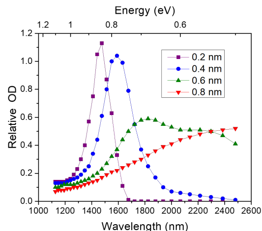
Fig. 3 A reproduction of theoretical calculations of the P3HT P1 polaron absorption band as a function of an anion distance from the P3HT chain, taken from Ref. 23; as the anion distance decreases from 0.8 nm to 0.2 nm, the P1 peak shifts towards smaller wavelengths and narrows significantly. 23 The calculations used a 10-mer of P3HT with a point-charge counteranion situated at the given distance away from the center of the polymer chain, along with a dielectric constant and a Huang-Rhys parameter of 1.0. 23 The vibrational frequency was chosen to be 0.17 eV, the intrachain coupling as -0.4 eV, the Gaussian disorder width as 0.3 eV, and the homogeneous linewidth to be 0.03 eV. 23 See Ref. 23 for details.
