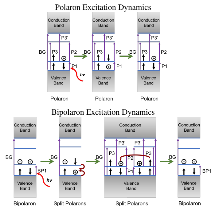
Fig. 4 Band diagrams explaining the dynamics expected following photoexcitation of polarons (top) and bipolarons (bottom) in the traditional conjugated polymer electronic structure picture; time flows from left to right. Following excitation of the low-energy polaron P1 transition, an electron is removed from the valence band and used to fill the pre-existing hole, creating a half-filled lower state and a filled P1 state. After rapid relaxation around the new hole, the system returns to the original ground-state polaron configuration. In contrast, when the BP1 transition of bipolarons is excited, an electron is taken from the valence band and used to fill one of the two holes, creating two single polarons in half-filled orbitals in different locations in the film. After any fast relaxation processes are complete, the two separated polarons must diffuse back together to reform the equilibrium bipolaron state, a process that is expected to occur on longer timescales.
