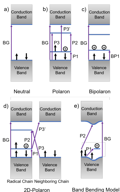
Fig. 2 a) The band diagram for neutral semiconducting polymers, which shows only a single optical transition (labeled BG); b) the traditional, longstanding electronic structure model for polarons in semiconducting polymers and their corresponding optical transitions. The P3 and P3' transitions are usually believed to be optically forbidden; c) the traditional model for bipolarons and their allowed BP1 optical transition; d) the model for 2-D-delocalized polarons, where optical transitions can occur both on the chain containing the majority of the radical cation character as well as diagonally between that chain and a neighboring, predominantly neutral chain. This makes the P3 and P3' transitions become optically allowed and breaks their degeneracy; e) a new band-bending model for the electronic structure of polarons on conjugated polymers that does not predict that a positively-charged polymer chain is easier to ionize than a neutral polymer chain. 19 There are no bipolarons or P3 or P3' transitions in this model.
