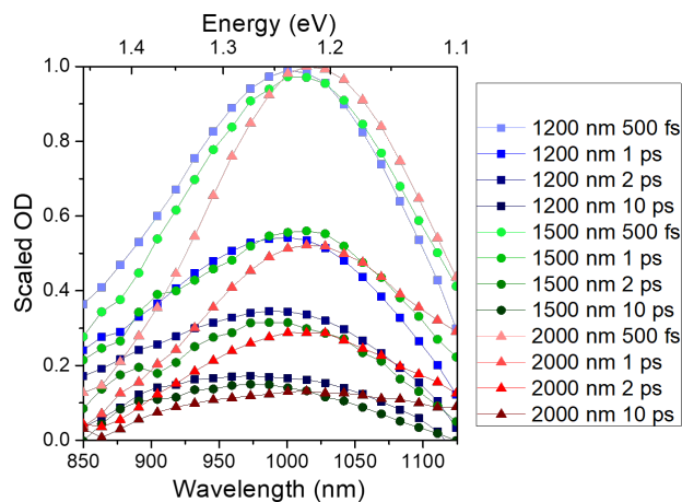
Fig. 6 Ultrafast transient absorption spectra of a P3HT film sequentially doped with a 1 mg/mL F4TCNQ solution in DCM following excitation at either 1200 nm (blue squares), 1500 nm (green circles) or 2000 nm (red triangles). Data are shown at 0.5, 1, 2, and 10 ps delays between excitation and collection, with darker colors used for later delay times. The observed transient absorption feature shifts to the blue, with the blue feature decaying more slowly, as the excitation wavelength is tuned to the blue.
