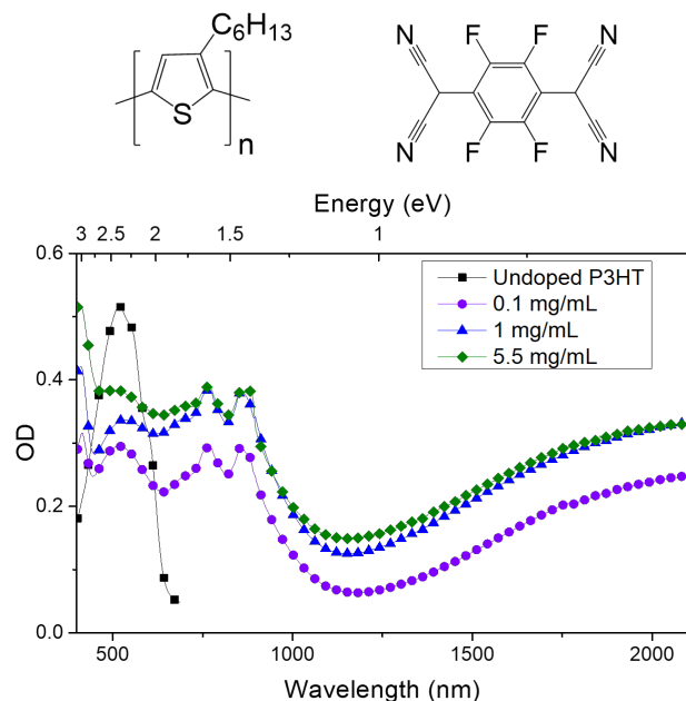
Fig. 1 Top Right: Chemical structure of the dopant F4TCNQ (2,3,5,6-tetrafluoro-7,7,8,8-tetracyanoquinodimethane. Top Left: Chemical structure of P3HT (poly(3-hexylthiophene-2,5-diyl)). Lower Panel: Steady-state UV-Vis-NIR absorption spectra of: an undoped P3HT film (black squares); an identical P3HT film after sequential doping using a 5.5-mg/mL solution of F4TCNQ in 70:30 THF:DCM (green diamonds); an identical P3HT film sequentially doped with a 1 mg/mL solution of F4TCNQ in DCM (blue triangles); and an identical P3HT film sequentially doped using a solution that was 0.1 mg/mL F4TCNQ in DCM (purple circles).
