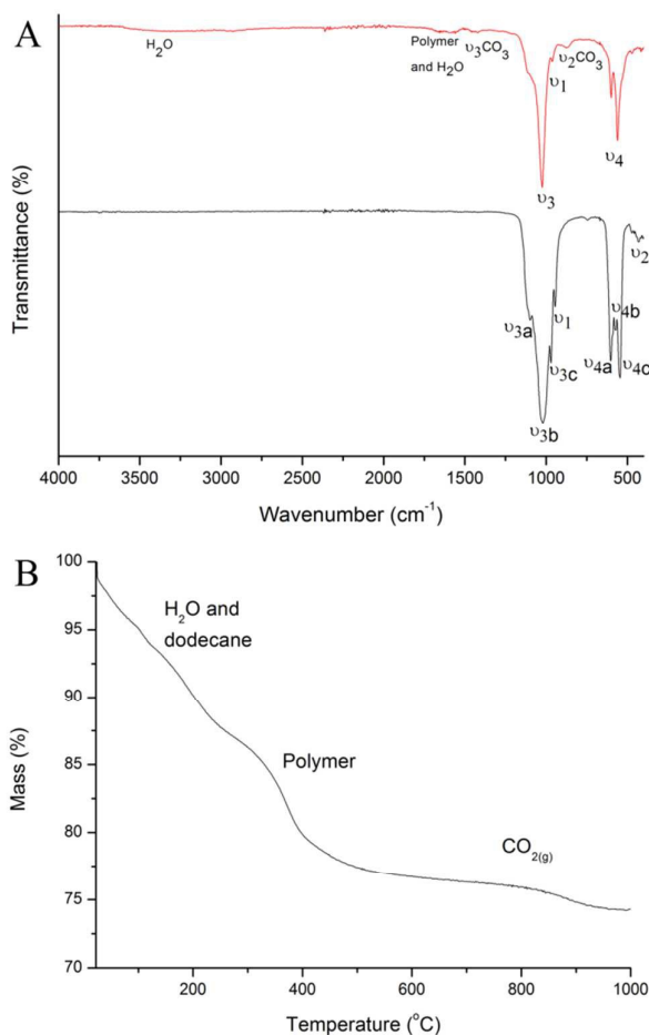
Fig. 3 (A) FTIR spectra of CaP capsules (red line), and CaP capsules annealed at 1000 °C (black line). (B) TGA curve of CaP capsules.
