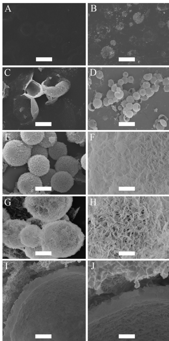
Fig. 2 SEM micrographs illustrating the mineralization of CaP at the surface of oil droplets stabilized with BCP. (A) Incubation periods of 0 hours (scale bar = 37 μm), (B) 48 hours (scale bar = 16 μm), (C) 60 hours (scale bar = 7 μm), (D and E) 72 hours (scale bars = 23 μm and 7 μm, respectively), (F) surface morphology of CaP capsule (scale bar = 704 nm), (G) CaP capsules annealed at 600 °C (scale bar = 2 μm), (H) surface morphology of CaP capsule after annealing at 600 °C (scale bar = 648 nm), and (I and J) shell thickness of the CaP capsules before annealing (scale bars = 1 μm and 540 nm, respectively).
