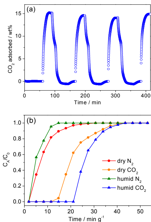
Fig. 5 (a) CO 2 adsorption-desorption cycling curve for 1-dmen in humid conditions. (b) Breakthrough curves for 1-dmen under dry (N 2 , red circle; CO 2 , orange circle) and wet conditions (N 2 , green triangle; CO 2 , blue triangle).
