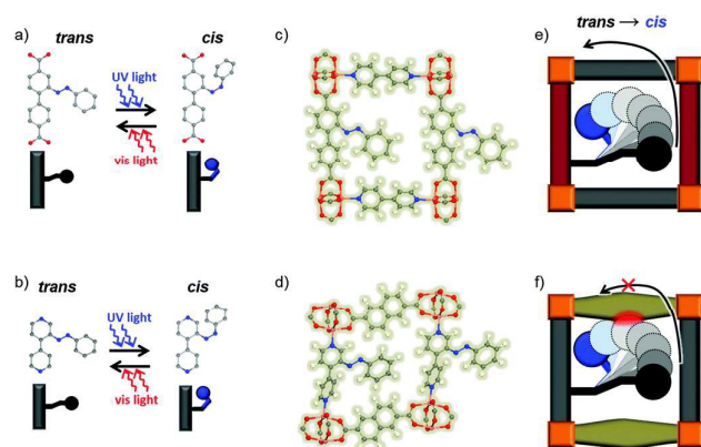
Figure 3. Changes in the pore dimensions of SURMOFs arising from the different linker lengths enable or disable the photoisomerization of azobenzene side-groups. Reference 28 – Published by the PCCP Owner Societies.
