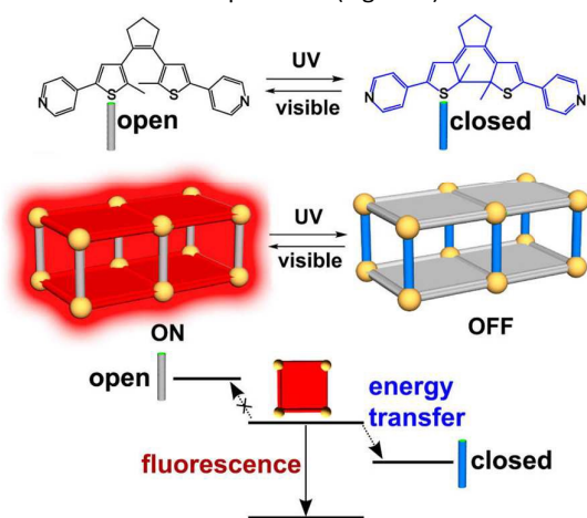
Figure 2. Energy transfer to the DTE-based linker in its closed form quenches fluorescence of the porphyrin-based linker. In this way, the MOF can be switched from an fluorescent to a non-fluorescent version by means of light. Reprinted with permission from reference 13. Copyright 2014 American Chemical Society.
