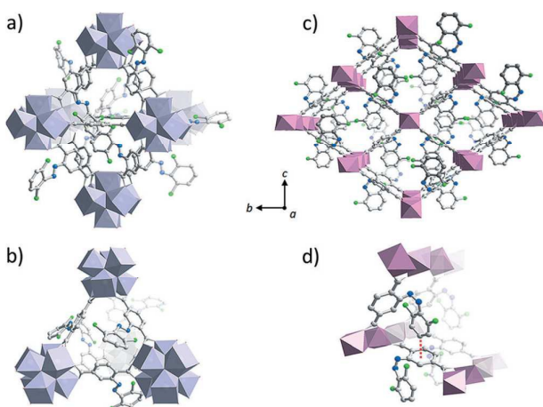
Figure 4. Terephthalic linkers featuring fluorinated azobenzene side-groups yielded a photochromic MOF isorecticular to UiO-66 (Zr) that switches E to Z upon green light irradiation and Z to E upon blue light exposure (a, b) and a MOF with similar to MIL-53(Al) with sterically crowded channels. The impossibility to isomerize in the last case gave place to a photothermal effect that decreased CO 2 sorption under visible light. Reprinted from reference 19 with permission from John Wiley and Sons.
