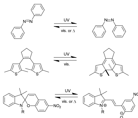
Scheme 1. Prototypical structures of photoswitchable molecular compounds: top, azobenzene (AB); center, dithienylethene (DTE); bottom, spiropyran/merocyanine (SP/MC).
