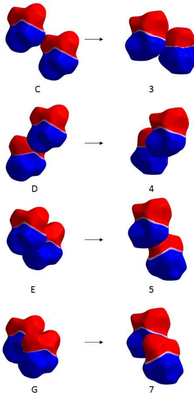
Figure 11: Changes in contacts C, D, E and G of \epsilon -glycine (shown on the left) on transformation to contacts 3, 4, 5 and 7 in \gamma -glycine (right) depicted using electrostatic potentials mapped onto Hirshfeld surfaces. Colour scheme as Fig. 4.
