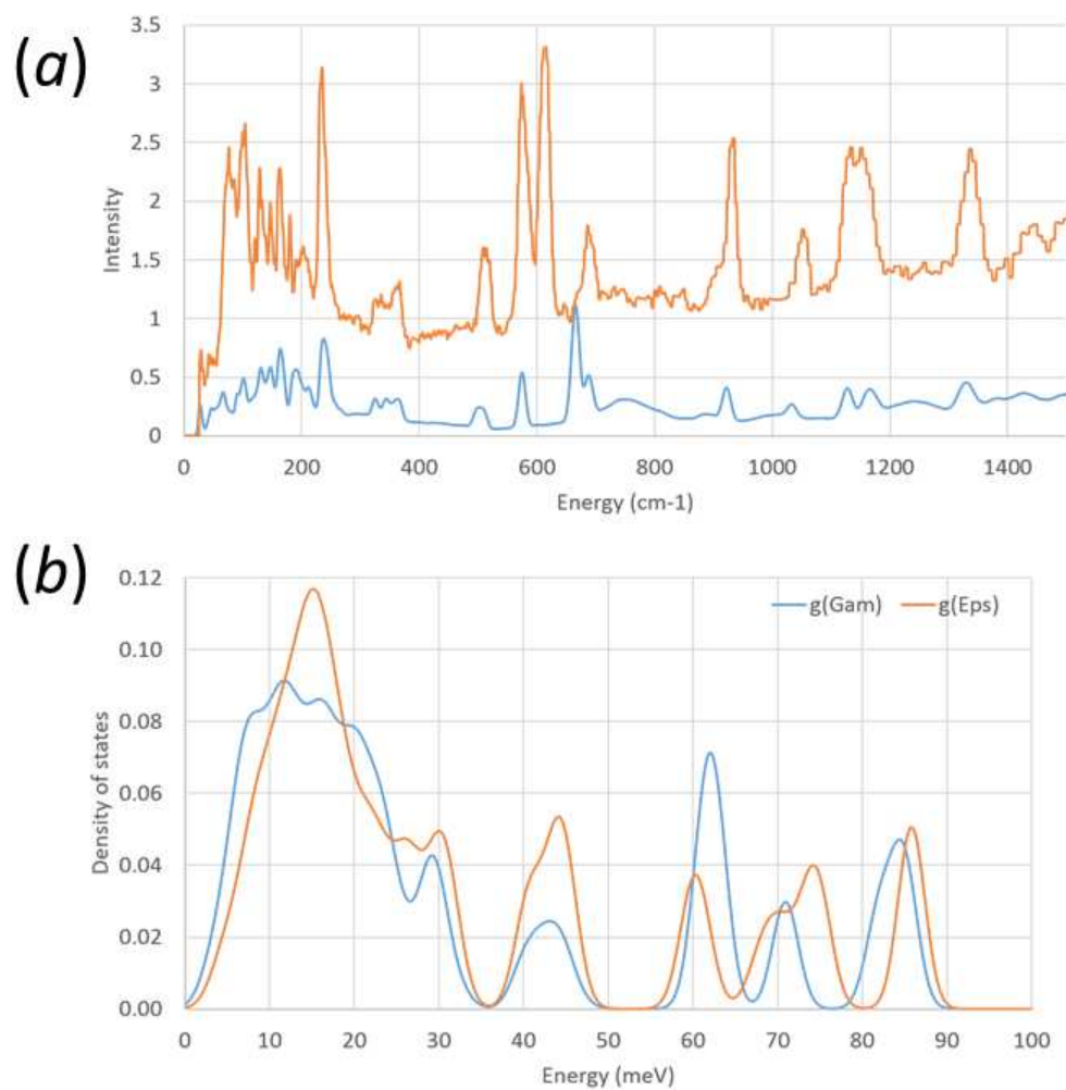
Figure 2: (a) Comparison of observed (red) and calculated (blue) phonon densities of states for \gamma -glycine- h_5 . (b) Calculated density of states for \gamma -glycine- h_5 (blue) and \epsilon -glycine- h_5 (red).
