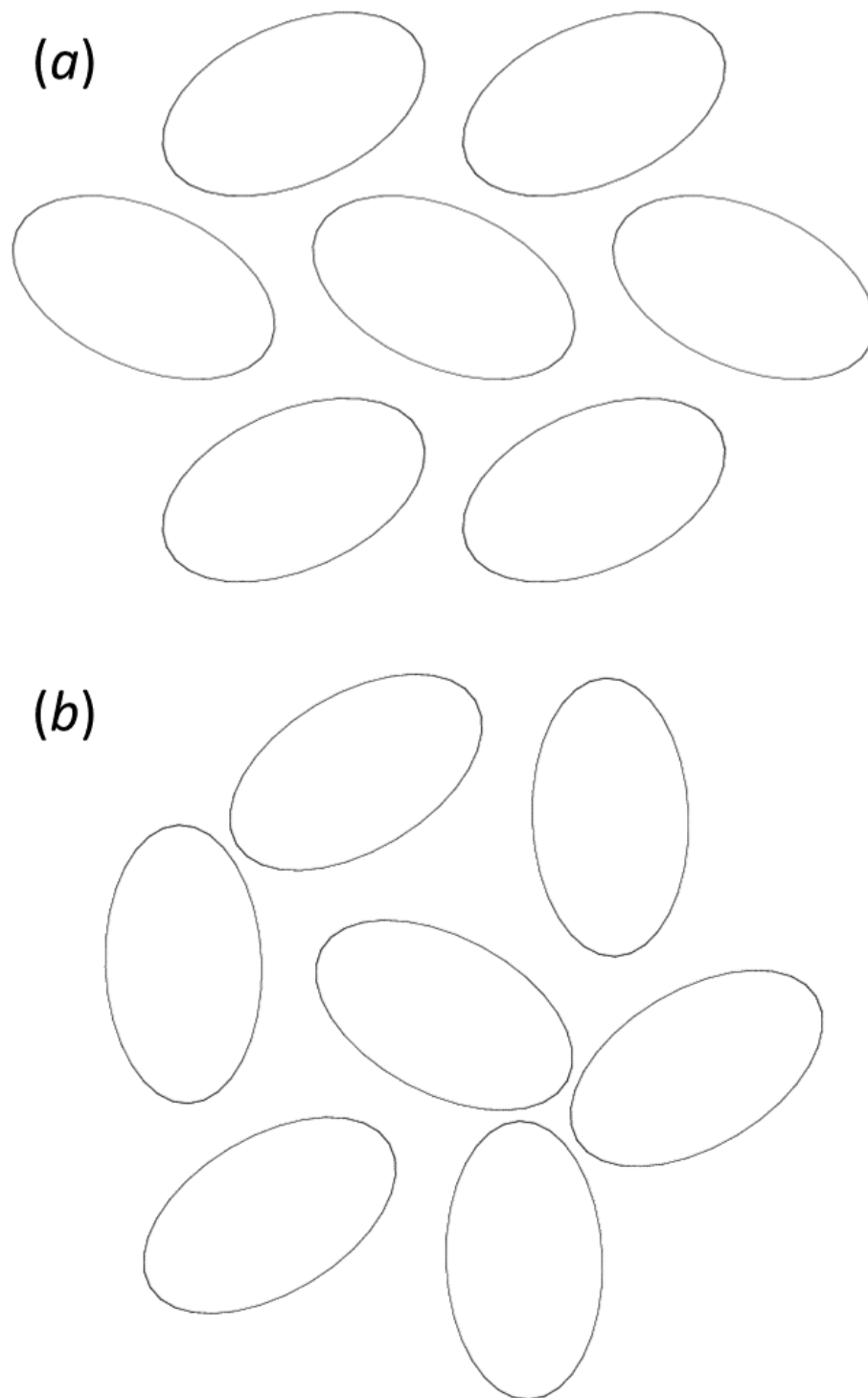
Figure 7: (a) \epsilon -glycine projected along [001] with molecules shown as inertial tensors. (b) The corresponding view for \gamma -glycine, also viewed along [001]. Both figures are on the same scale.
