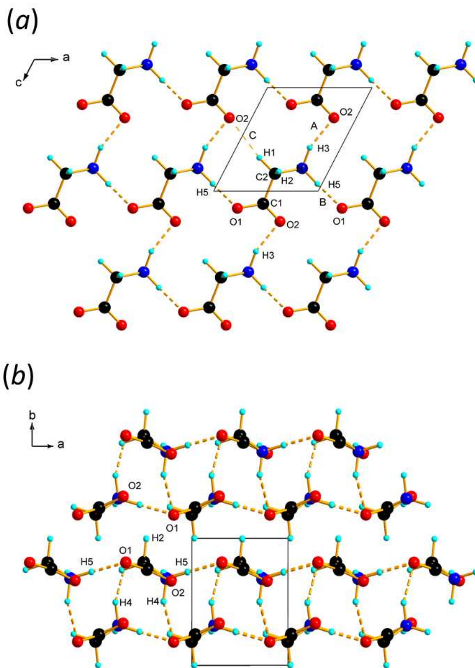
Figure 3: (a) Layers formed parallel to the ac planes in \epsilon -glycine at 4.3 GPa. (b) Stacking of layers along b .
