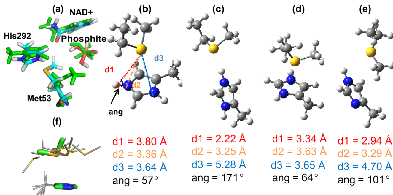
Figure 3. (a) Representative structures of the interaction between Met53 and the QM region at the intermediate (Int, green atoms) and at the transition state for the hydride transfer step (TS2, atoms coloured by atom type) from AM1/CHARMM27 calculations. (b)–(e) Structures of complexes of 4-methyl imidazole/imidazolium and methylthioethane fragments (representing His and Met) optimized at the MP2/6-31+G(d) level unless otherwise stated. (b) The average AM1/CHARMM27 (QM/MM) TS2 structure of the 4-methyl imidazolium and methylthioethane fragments (averaged over 110 snapshots at the reaction coordinate window for TS2). (c) Hydrogen-bonded complex between 4-methylimidazolium and methylthioethane. (d) Face-on complex between 4-methylimidazolium and methylthioethane. (e) Neutral complex between 4-methylimidazole and methylthioethane. (f) The structural template for the His-Met interaction search shown in sticks (green carbons) superimposed (on His atoms only) with the 10 hits from the Protein Data Bank with the lowest RMSD (grey carbons). As indicated in (b) d1 is the S \delta –He separation, d2 is the S \delta –Ne distance, d3 is the S \delta –N \delta distance and ang is the Ne–He–S \delta angle.
