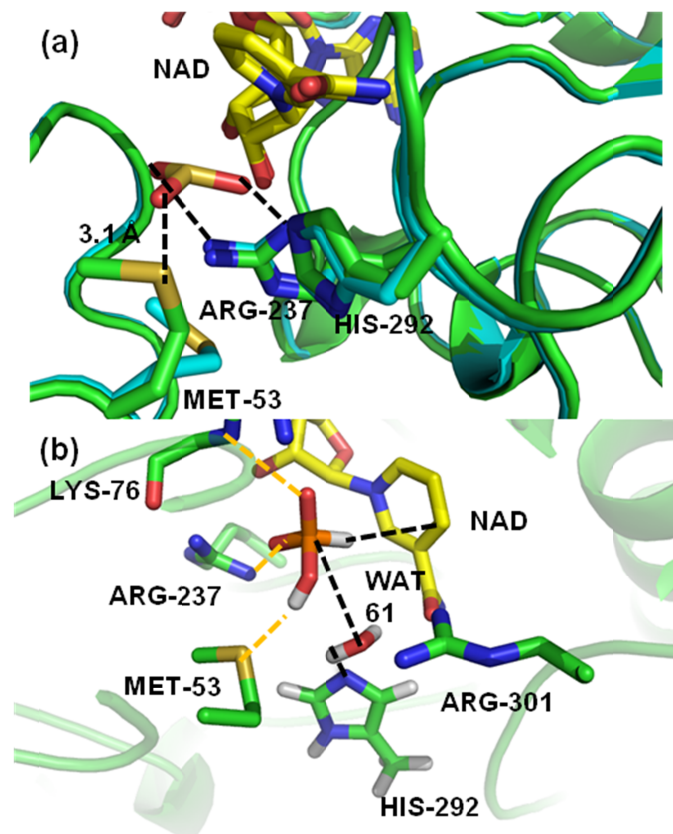
Figure 2 (a) A representation of the crystal structures of the most stable TS-PTDH with the \text{NAD}^+ co-factor and sulfite inhibitor 11 in green and the complex without sulfite in blue. \text{NAD}^+ (shown with yellow carbons) and several key active site residues are shown as sticks and their interactions with the sulfite inhibitor are indicated by dotted lines. Arg237 is important for binding of the substrate and His292 is the putative base for the reaction. 6 When sulfite is present, the Met53 sulfur (S \delta ) to sulfite oxygen distance is 3.1 Å. In the absence of sulfite, the side chain of Met53 adopts a different orientation. (b) A representative snapshot of the PTDH ternary complex from QM/MM MD simulations showing important interactions in the active site. The black dotted lines indicate the distances involved in the reaction coordinate.
