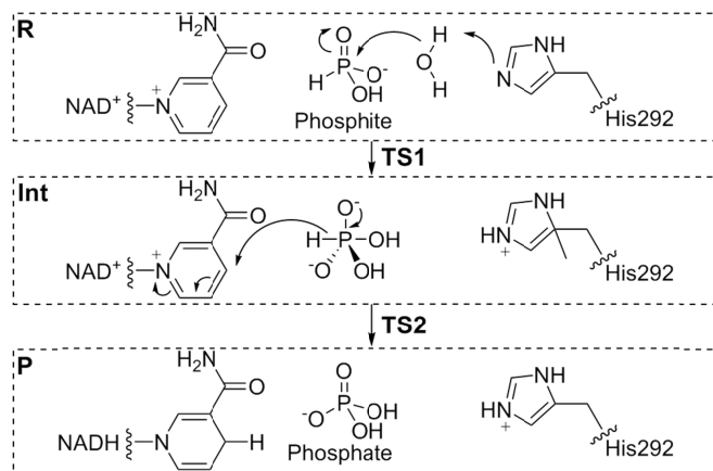
Figure 1. An associative mechanism, as modelled here, for the nucleophilic displacement reaction catalysed by PTDH, with His292 as the base. 1 R = reactant state, Int = pentavalent intermediate, P = product. TS1 and TS2 are the transition states for the first and second steps.
