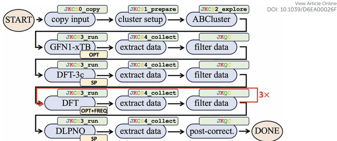
Figure 4. JKCS workflow proposed by Kubečka et al., 2023 39 . Adapted from ref. 39 with permission from the American Chemical Society, copyright 2023.
