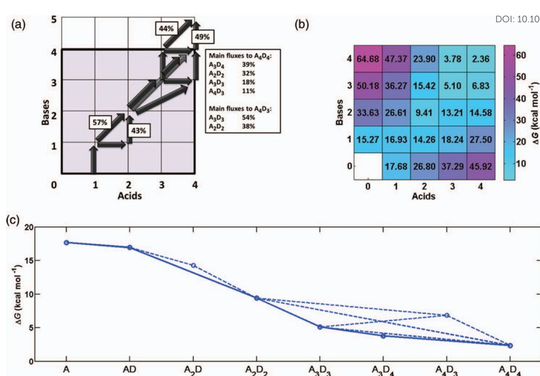
Figure 8. Main clustering pathways and Gibbs free energies of formation of the clusters in the electrically neutral sulfuric acid-DMA system at T = 5^\circ\text{C} , [\text{SA}] = 10^6 \text{ cm}^{-3} and [\text{DMA}] = 1 \text{ ppt} . Panel (a): Major routes leading out of the simulated system. For figure clarity, the arrows that fall on top of each other are colored with different shades. Panel (b): Formation free energies of a cluster in the system. Panel (c): formation free energy of the growing cluster as a function of growth step. Solid and dashed lines: correspond to the major and minor fluxes, respectively. Adapted from Olenius et al., 2013 76 . Reproduced from ref. 76 with permission from the AIP Publishing, copyright 2013.
