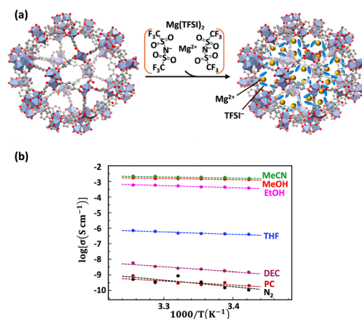
Fig. 4 (a) Structural illustration of \text{MIL-101} \cap \{\text{Mg}(\text{TFSI})_2\} , showing the incorporation of \text{Mg}^{2+} and \text{TFSI}^- within the framework pores. (b) Arrhenius plots of ionic conductivity for \text{MIL-101} \cap \{\text{Mg}(\text{TFSI})_2\} under various anhydrous vapors. Exposure to MeCN, methanol (MeOH), and ethanol (EtOH) vapors significantly enhances conductivity ( >10^{-3} \text{ S cm}^{-1} ), whereas tetrahydrofuran (THF), diethyl carbonate (DEC), propylene carbonate (PC), and dry \text{N}_2 result in poor conductivity. Adapted from ref. 49 with permission from the American Chemical Society, copyright 2022.
