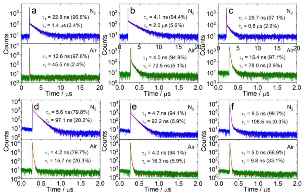
Fig. 3 Fluorescence decay traces of (a) PTZ-DTO at 560 nm, (b) PSeZ-DTO at 550 nm, (c) DPTZ-DTO at 580 nm, (d) PTZ-O-DTO at 400 nm, (e) PTZ-O 2 -DTO at 410 nm and (f) DPTZ-O-DTO at 470 nm under different atmospheres (N 2 and air). \lambda_{\text{ex}} = 340 nm, c = 1.0 \times 10^{-5} M in TOL, 25 °C.
