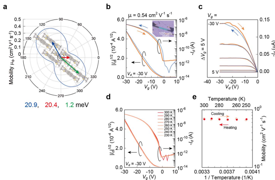
Fig. 3 Evaluation of MT-coronene as a semiconducting material. (a) Calculated t_s and estimated mobility based on the hopping model. (b) Transfer and (c) output characteristics of SC-FET of MT-coronene measured in air. (d) Transfer characteristics measured at various temperatures in a vacuum. (e) Temperature dependence of carrier mobility.
