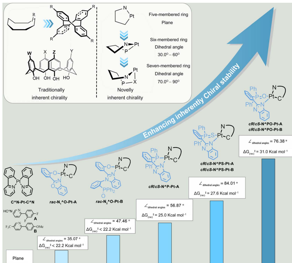
Fig. 1 The designed scheme and chemical structures of inherently chiral Pt(II) complexes ( \angle dihedral angles: angle between the phenyl plane and the PtC N coordination plane; \Delta G_{(rac)}^{\ddagger} : racemization energy barriers of inherently chiral Pt(II) complexes).
