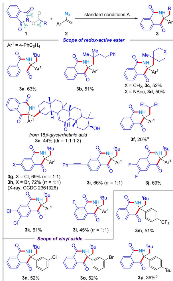
Fig. 2 Substrate scope for the photocatalytic two-component [4 + 2] reaction. Unless otherwise noted, the reaction was conducted under conditions 1 (0.18 mmol), 2 (0.10 mmol), Ir(ppy) 3 (bpy)PF 6 (2 mol%), Hantzsch ester (0.4 mmol), A1 (0.25 mmol) in DCM (0.56 M) irradiated with 30 W blue LEDs at 35 °C for 16 h. a The reaction was conducted using 4CzIPN (2 mol%), DIPEA (80 mol%), and DCM (1.0 mL). b HOAc (80 mol%) was added.
