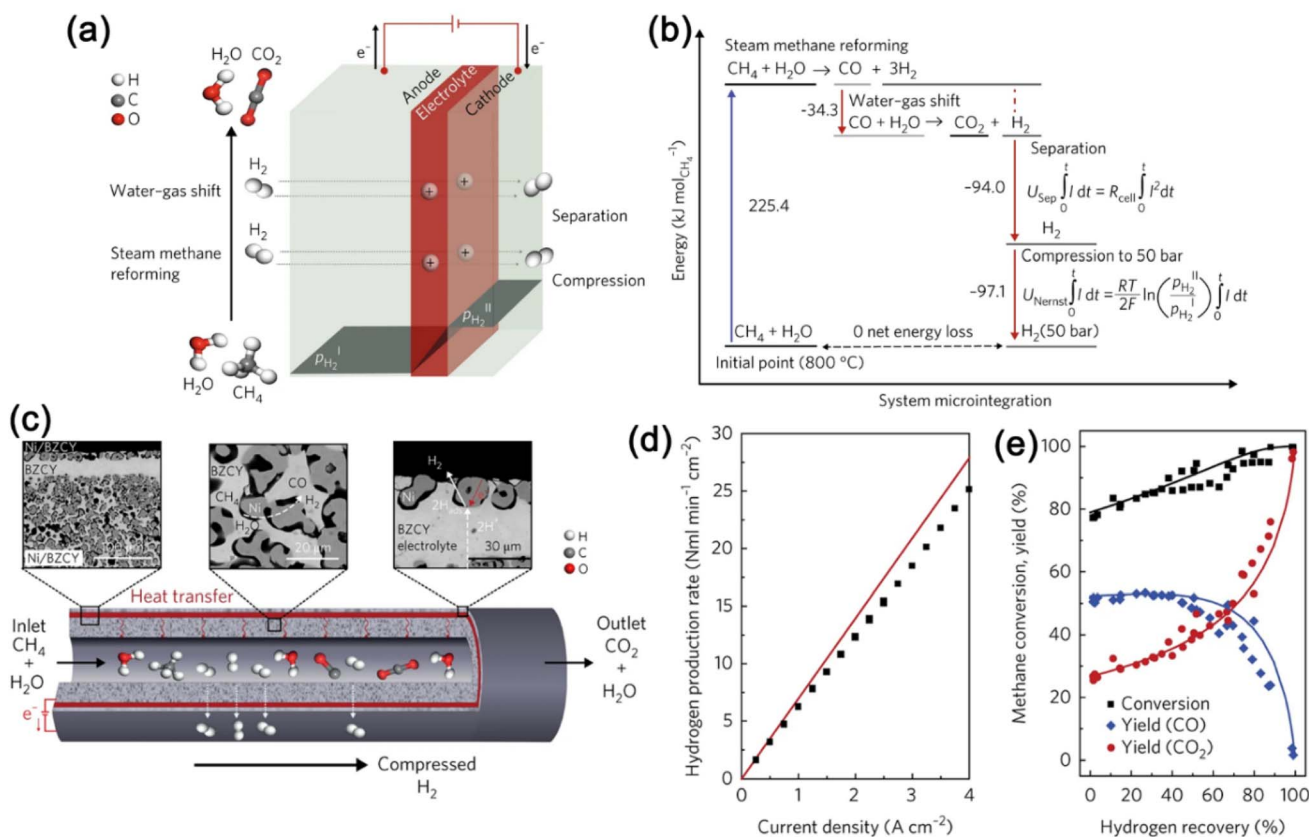
Fig. 24 (a) Schematic illustration of H-SEMRs integrated with an electro-chemical \text{H}_2 compression process, (b) energy balance and system micro-integration for operation at 800^\circ\text{C} for a feed inlet of one mole \text{CH}_4 , (c) tubular SEMRs with Ni catalyst loaded inside the ceramic tube (insets are SEM cross-section images of the overall cell and electrode reactions), (d) \text{H}_2 production rate versus current density compared with the theoretical value and (e) conversion, yield of \text{CO}_2 and \text{CO} versus hydrogen recovery at 800^\circ\text{C} , 10 bar, \text{S/C} = 2.5 . Steam pressure on the hydrogen side inlet was 0–2.0 bar. Reproduced with permission from ref. 274.
