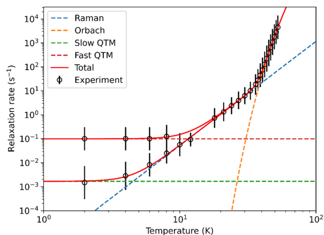
Fig. 4 Fitting of 1-Dy relaxation profile, showing Orbach, Raman and QTM components derived from eqn (S5).† Error bars represent one ESD in the distribution of rates.
