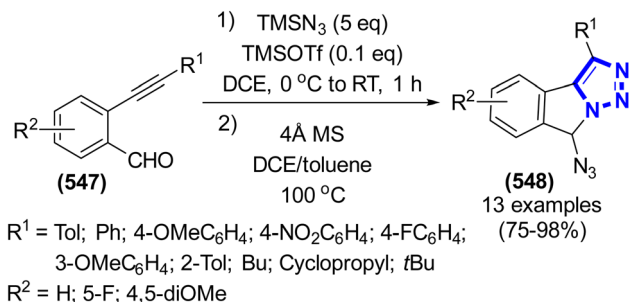
Scheme 145 Synthesis of 1,2,3-triazole-fused isoindoles catalyzed by \text{TMSOTf} .
