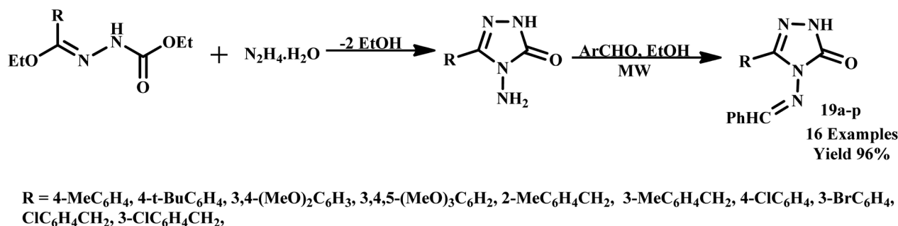
Scheme 13 Synthetic route of 3-aryl-4-arylmethylideneamino-4,5-dihydro-1H-1,2,4-triazol-5-ones (19a-p). 48
