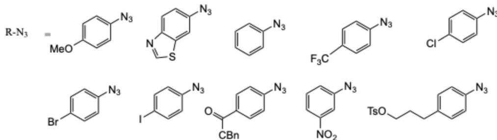
Scheme 62 Microwave-assisted synthesis of 1,2,3-triazoles (73a–k). 109
