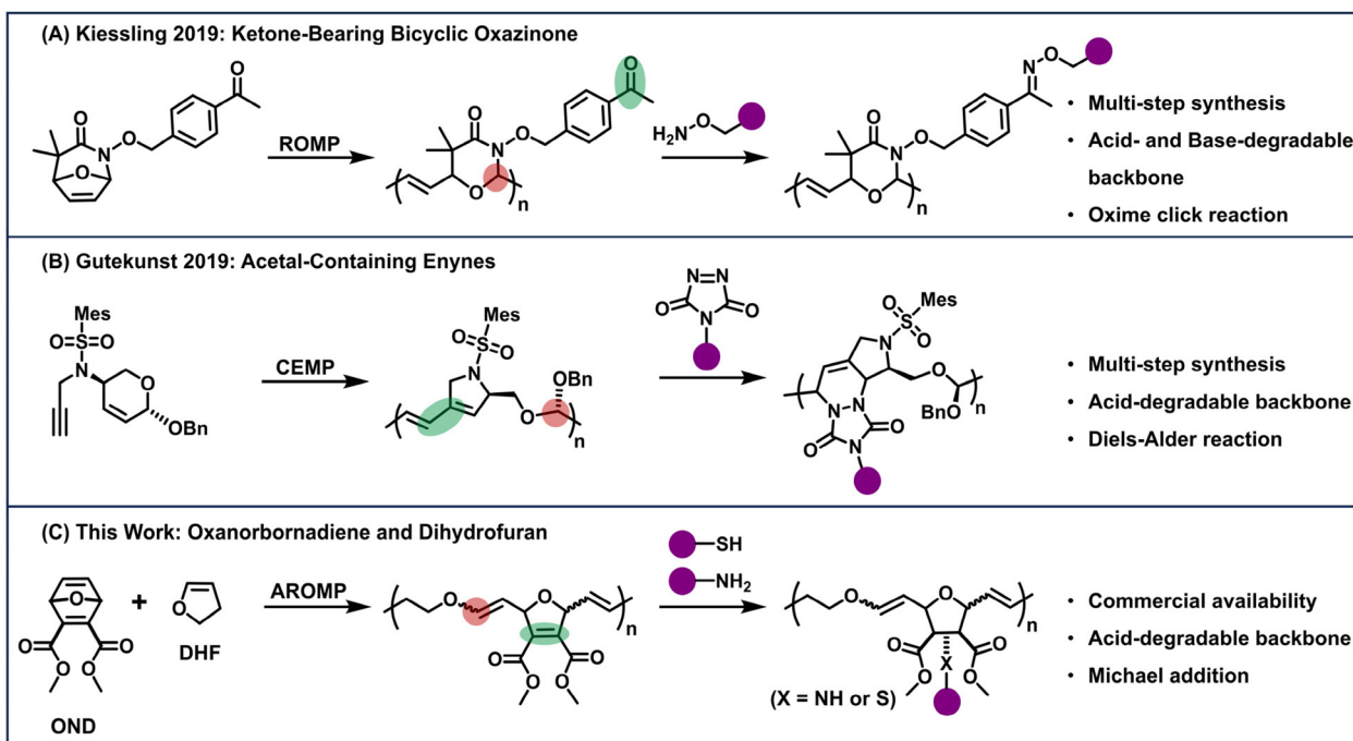
Fig. 1 Degradable and functionalizable polymers via olefin metathesis polymerization strategy. (A) ROPM of ketone-bearing bicyclic oxazinone followed by an oxime click reaction. (B) Cascade enyne metathesis polymerization (CEMP) of acetal-containing enyne monomers, followed by Diels–Alder reaction. (C) This work: alternating ring-opening metathesis copolymerization (AROMP) of oxanorbornadiene dicarboxylate and 2,3-dihydrofuran. The resulting polymers are capable of post-polymerization modification via Michael addition.
