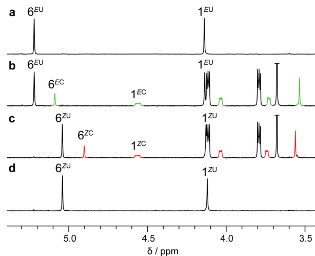
Fig. 4 Stacked partial ^1H NMR (500 MHz, CD_3CN , 298 K, 1.4 mM) spectra of (a) axle EE-4H^+ , (b) a 1 : 1 mixture of EE-4H^+ and crown ether 2 , (c) the same sample after exhaustive irradiation at 365 nm and (d) axle ZZ-4H^+ .
