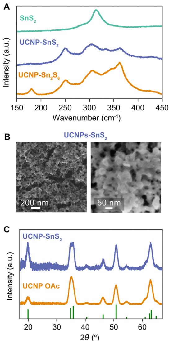
Fig. 5 Annealing Sn 2 S 6 4- -capped 9-nm NaYF 4 : 8% Tm 3+ UCNPs at 350 °C to form a UCNP-SnS 2 nanocomposite. (A) Raman spectra of the Sn 2 S 6 4- -capped UCNPs before (orange line) and after (blue line) annealing. Also shown is the spectrum of the SnS 2 matrix formed by annealing Na 4 Sn 2 S 6 (green line). (B) SEM images of the UCNPs embedded in the SnS 2 matrix. (C) X-ray diffraction spectra of the UCNPs-SnS 2 nanocomposite (blue line) and oleate-capped UCNPs (orange line). The reference spectrum for hexagonal-phase NaYF 4 (PDF# 04-022-5333) is also shown (green line).
