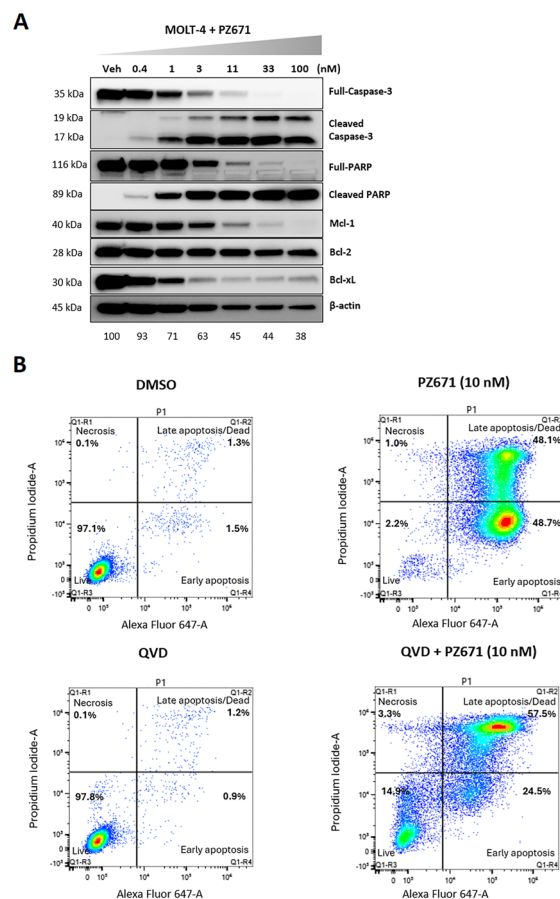
Fig. 5 Characterization of PZ671-mediated apoptosis in MOLT-4 cells. (A) Western blot analysis of cleaved PARP and cleaved caspase-3 after 16 h of treatment with indicated concentrations of PZ671. The full-PARP blot was from the stripped membrane and re-probed with cleaved PARP, resulting in the rectangular shape. Percentage decrease in \beta -actin levels due to toxicity was normalized to the control sample. (B) Flow cytometry analysis of apoptosis using annexin V and PI staining. MOLT-4 cells were treated with PZ671 at 10 nM for 24 h. PZ671 significantly increased the percentage of apoptotic cells and QVD (10 \mu M) pretreatment for 2 h inhibited the apoptosis induced by PZ671. Data are representative of two independent experiments.
