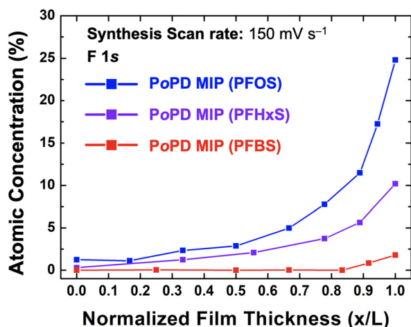
Fig. 8 Normalized XPS SDP of the F 1s signal for the representative MIP films imprinted with PFOS, PFHxS, and PFBS at the same synthesis scan rate of 150 mV s -1 . Values are the averaged values from separate measurements ( N \geq 3 ).
